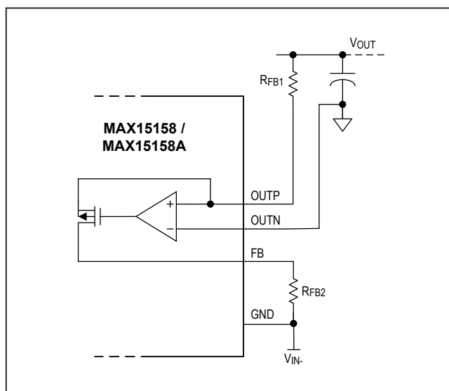
Figure 1. Using Internal FB Level Shifter
